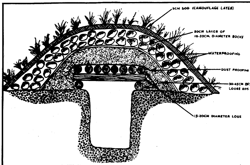
Figure 4-34. Overhead Cover.
