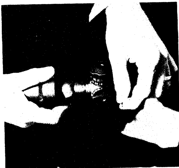
Figure 3-17. Zeroing with Allen Wrench Windage Control (View 1).
